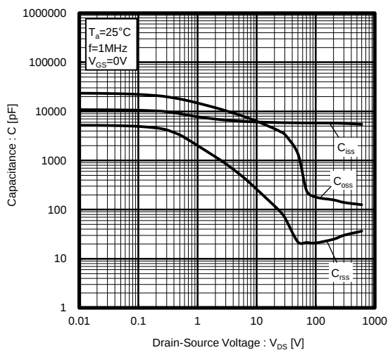
Fig.11 Typical Capacitance vs. Drain-Source Voltage
