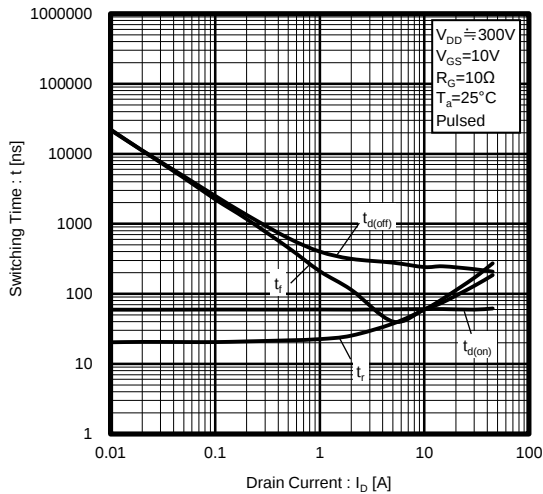
Fig.9 Switching Characteristics
