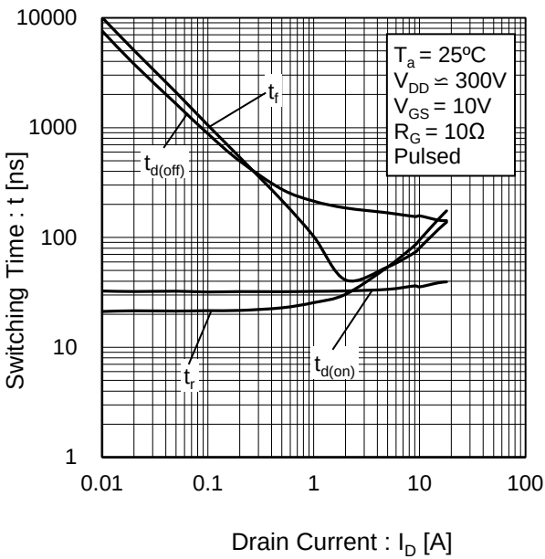
Fig.20 Switching Characteristics
