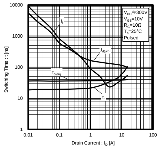
Fig.10 Switching Characteristics
