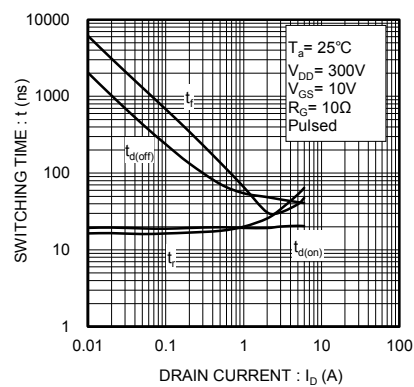
Fig.14 Switching Characteristics
