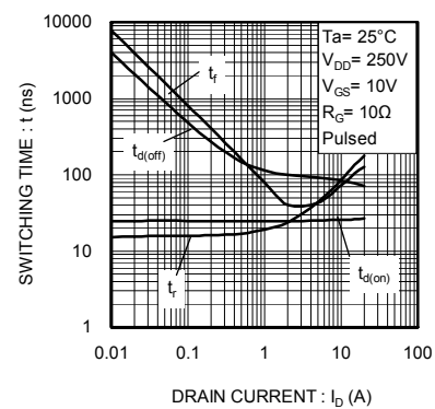
Fig.14 Switching Characteristics
