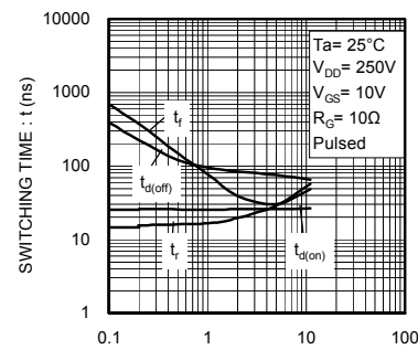
Fig.14 Switching Characteristics
