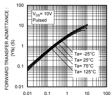
Fig.9 Forward Transfer Admittance vs. Drain Current
