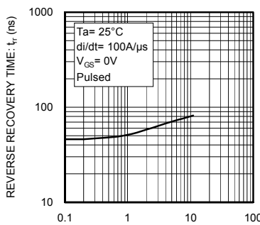
Fig.13 Reverse Recovery Time vs. Reverse Drain Current
