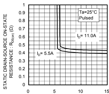
Fig.7 Static Drain-Source On-State Resistance vs. Gate Source
