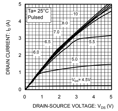
Fig.3: Typical Output Characteristics( II )
