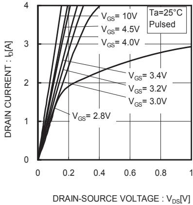
Fig.1 Typical Output Characteristics(I)
