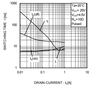
Fig.11 Switching Characteristics
