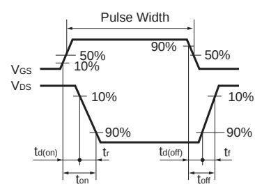
Fig.1-2 Switching Waveforms
