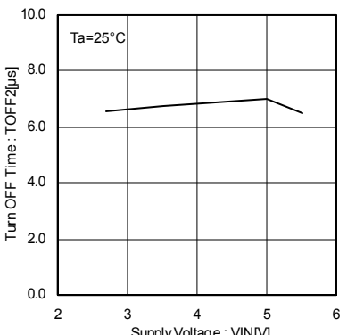
Fig.25 Output turn-off time
