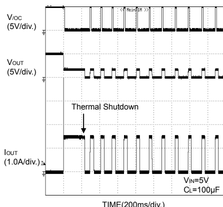
Fig.36 Thermal shutdown 1Ω load connected at enable
