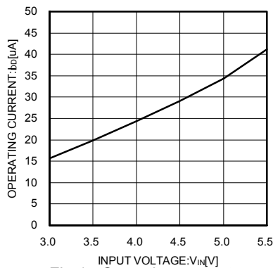
Fig.14 Operating current
