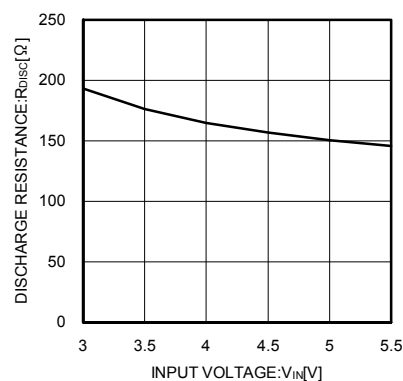
Fig.19 Discharge resistance
