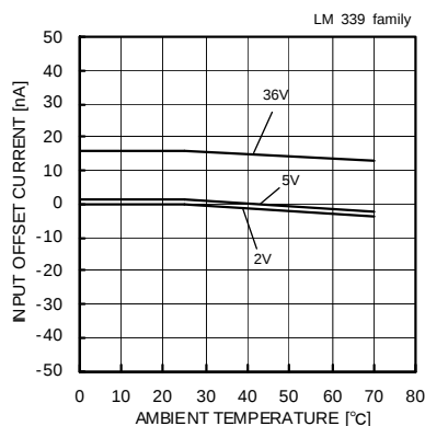
Fig. 33 Input Offset Current – Ambient Temperature
