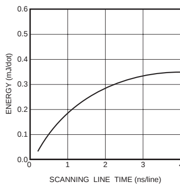
Fig.3 Maximum energy curve
