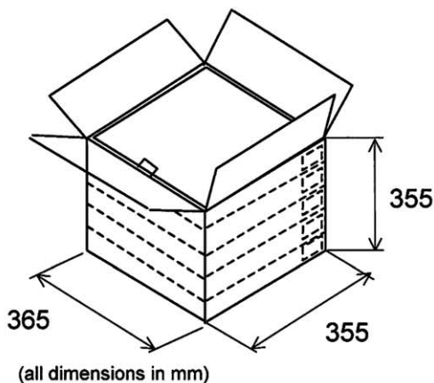
Fig. 7 Shipping box dimensions and Shipping style
