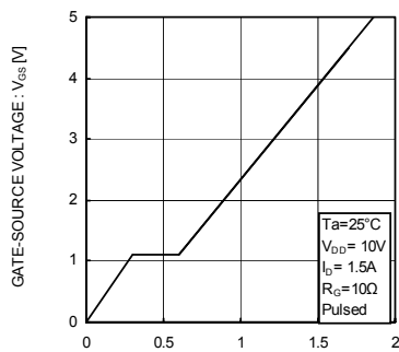
Fig. 13 Dynamic Input Characteristics
