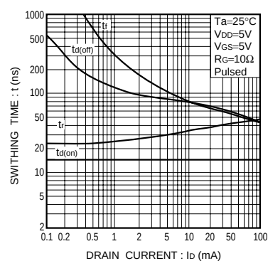
Fig.20 Switching characteristics
