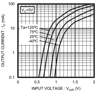
Fig 3. Output Current vs. Input Voltage (OFF Characteristics)
