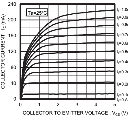
Fig 1. Output Current vs. Output Voltage
