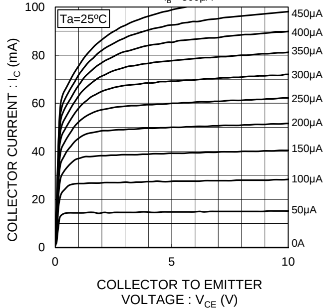
Fig.2 Grounded emitter output characteristics I_B = 500\mu A
