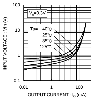
Fig.2 Input Voltage vs. Output Current
