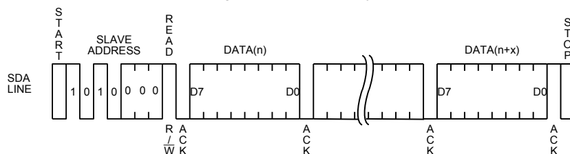
Fig.37 Current read cycle
