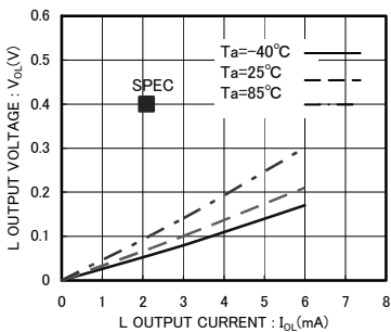
Fig.6 'L' output voltage V_{OL-I_{OL}} ( V_{CC}=1.7V )
