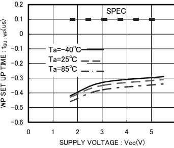
Fig.30 WP setup time t_{SU : WP}
