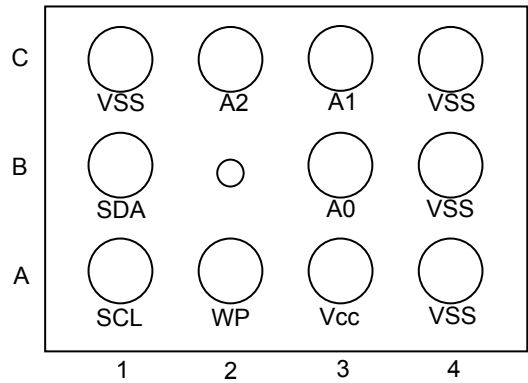
Fig.3 BU9897GUL-W(bottom view)
