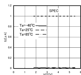
Fig.10 Input leak current I_{LI} (CS,SK,DI)
