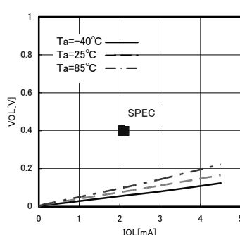
Fig.6 L output voltage V_{OL} - I_{OL} ( V_{CC} = 4.0\text{V} )
