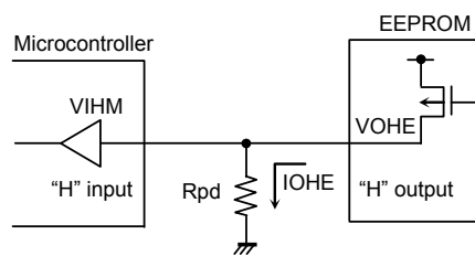
Fig.47 DO pull down resistance
