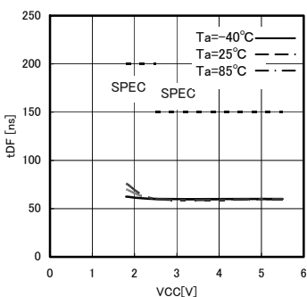
Fig.28 Time from CS to High-Z tDF
