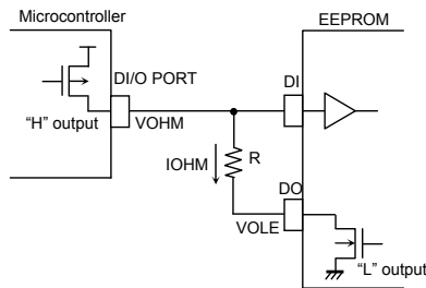
Fig. 53 Circuit at DI, DO direct connection (Microcontroller DI/O "H" output, EEPROM "L" output)
