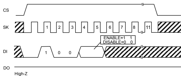
Fig.35 Write enable (WEN) / disable (WDS) cycle
