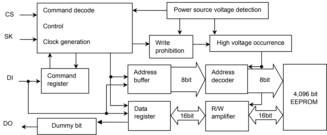
Fig.30 Block diagram
