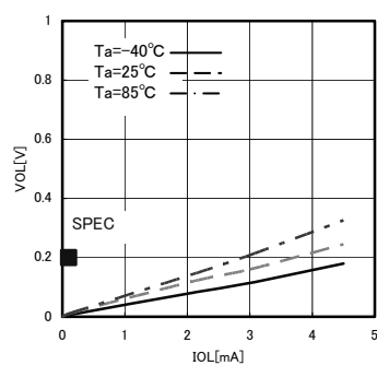
Fig.5 L output voltage V_{OL} - I_{OL} ( V_{CC} = 2.5\text{V} )
