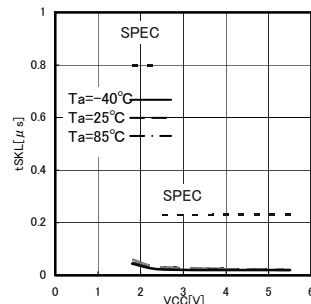
Fig.19 SK low time tSKL
