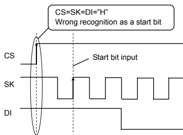
Fig.38 Wrong action timing
