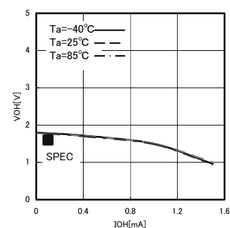
Fig.7 H output voltage V_{OH} - I_{OH} ( V_{CC} = 1.8\text{V} )
