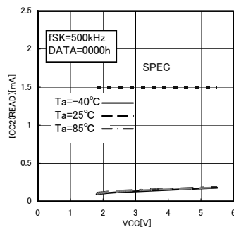
Fig.15 Consumption current at READ action ICC2 (READ, fSK=500kHz)
