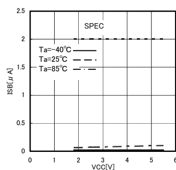
Fig.16 Consumption current at standby action ISB
