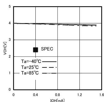
Fig.9 H output voltage V_{OH} - I_{OH} ( V_{CC} = 4.0\text{V} )
