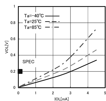
Fig.4 L output voltage V_{OL} - I_{OL} ( V_{CC} = 1.8\text{V} )
