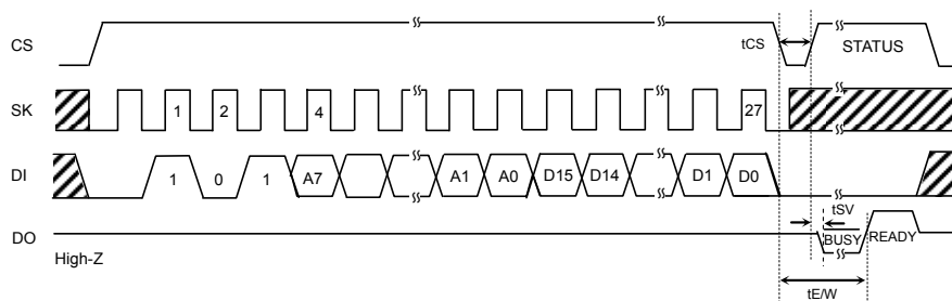
Fig.34 Write cycle
