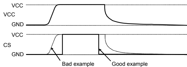
Fig.55 Timing at power ON/OFF
