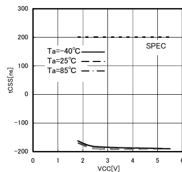
Fig.22 CS setup time tCSS
