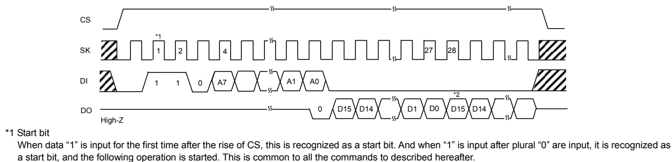
Fig. 33 Read cycle
