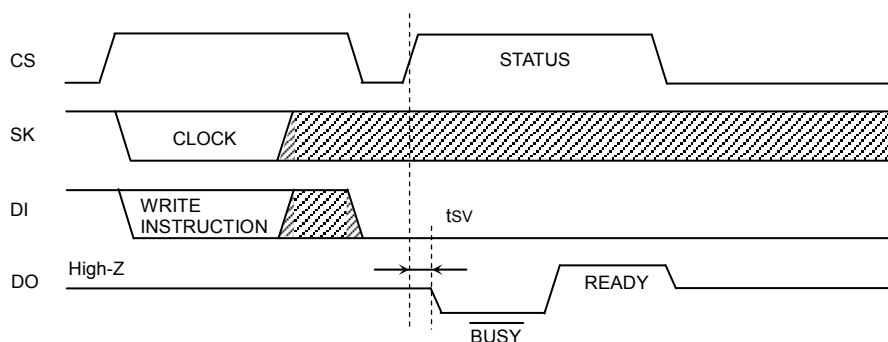
Fig.41 R / \overline{\text{B}} status output timing chart
