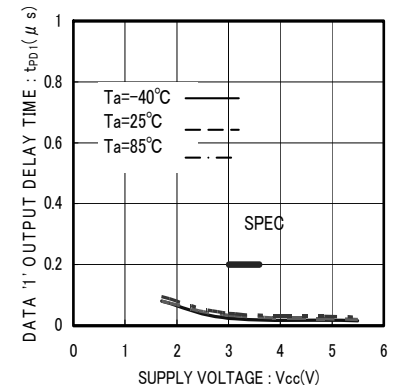
Fig.19 Data '1' output delay time t_{PD1}
