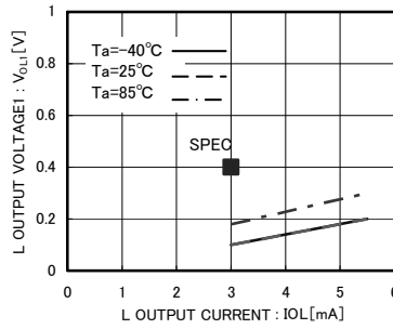
Fig.11 'L' Output Voltage1 V_{OL1-IOL} ( V_{CC1}=3.0V ) (SDA1)
