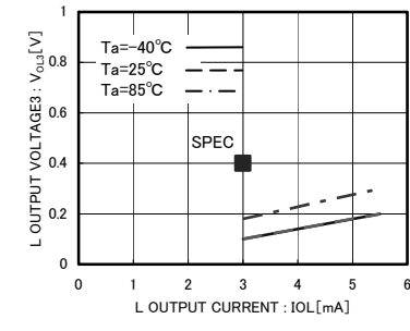
Fig.13 'L' Output Voltage3 V_{OL3-IOL} ( V_{CC3}=3.0V ) (SDA3)
