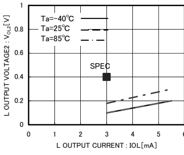
Fig.12 'L' Output Voltage2 V_{OL2-IOL} ( V_{CC2}=3.0V ) (SDA2)
