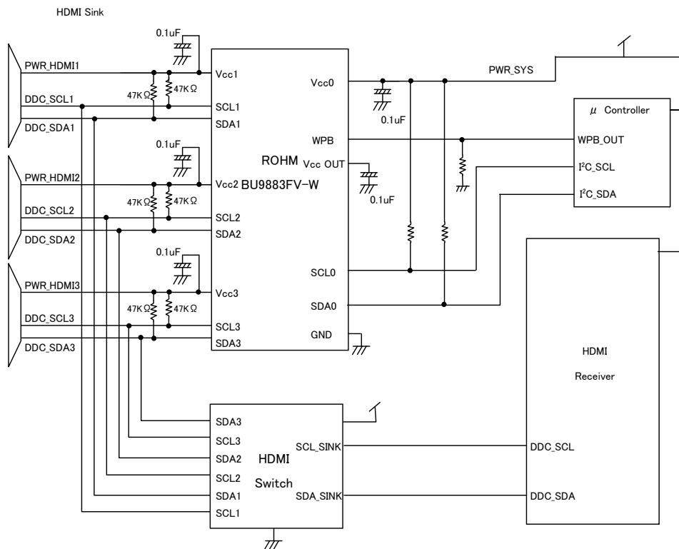
Fig.39 Application circuit
