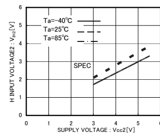
Fig.4 'H' Input Voltage2 V_{IH2} (SCL2,SDA2)
