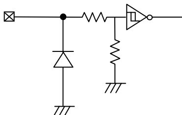
Fig.60 Input pin circuit diagram
