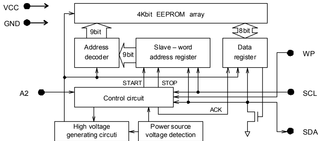
Fig.2 Block diagram
