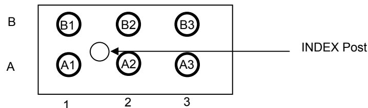
Fig.3 BU9847GUL-W(bottom view)
