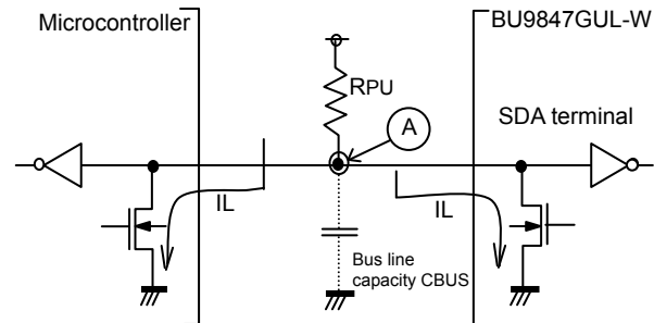
Fig.47 I/O circuit diagram
