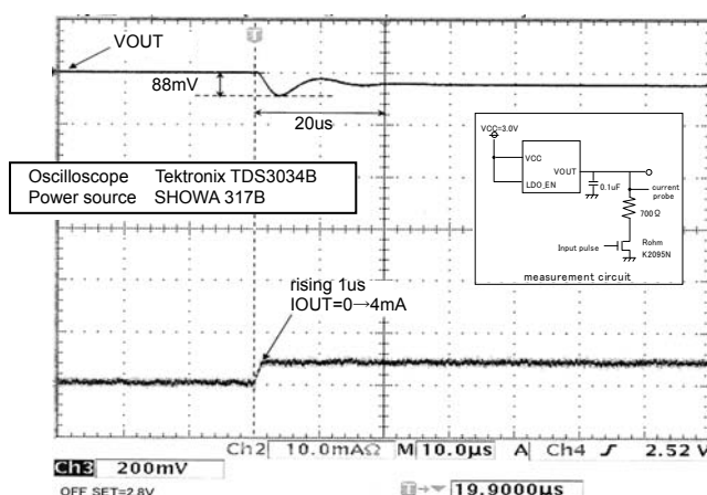
BU9829GUL-W Evaluation result ( I_{OUT}=0\text{mA}\rightarrow 4\text{mA} , C_{OUT}=0.1\mu\text{F} )
