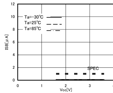
Fig.15 Standby operation ISB (EEPROM)
