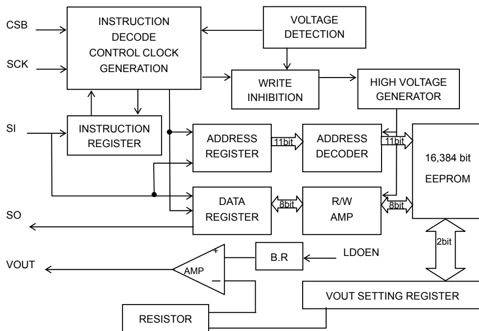
Fig.6 Block diagram
