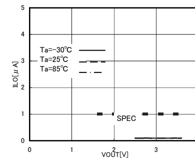
Fig.12 Output leak current ILO
