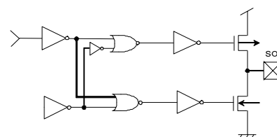
Fig.49 SO terminals equivalent circuit
