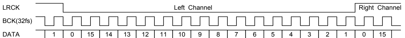
Figure 5.12.1 I2S Output Timing (32fs)
