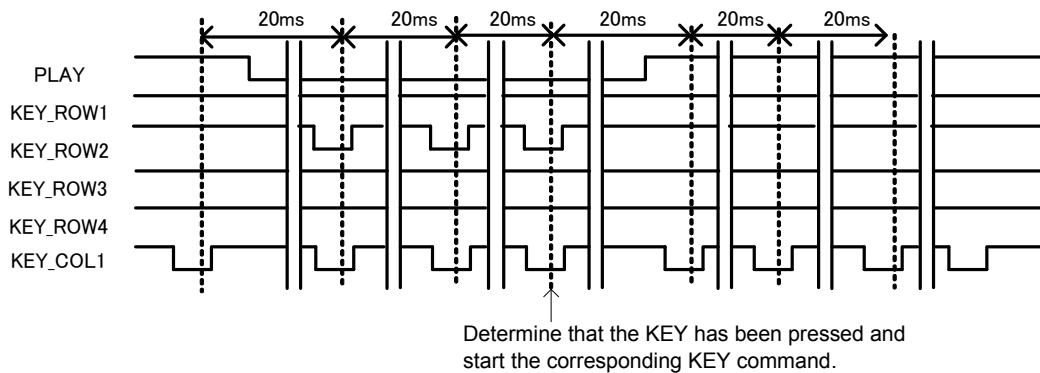
Figure 6.3.2 Operation Waveforms when KEY is Pressed
