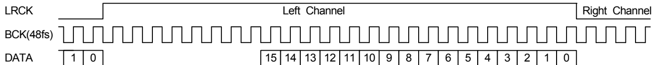
Figure 5.21.1.2 EIAJ Input Timing (48fs)
