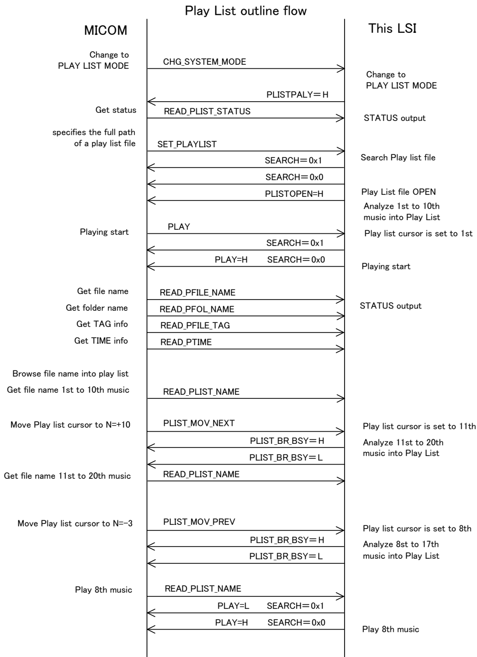
Figure 6.4.8.1 Play List playing outline flow
