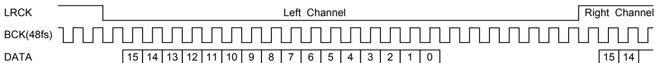
Figure 5.12.2 I2S Output Timing (48fs)
