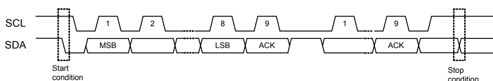
Figure 5.15.1 I2C Start and Stop Conditions
