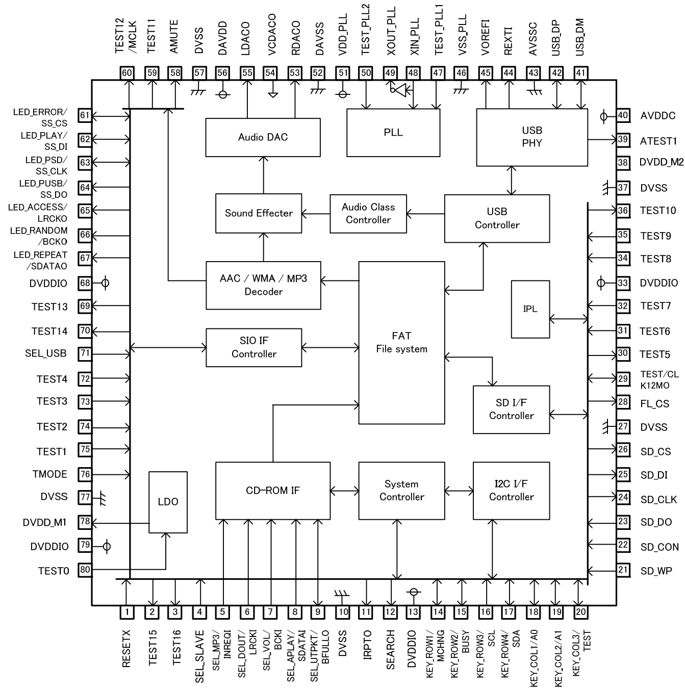
Block diagram
