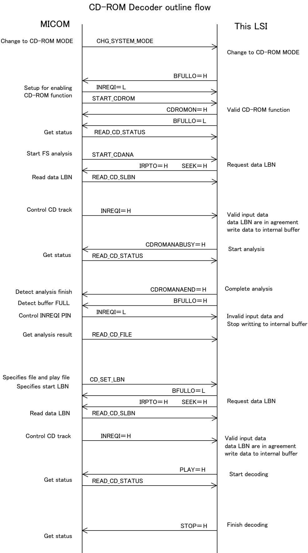
Figure 6.4.10.1 File read function outline flow
