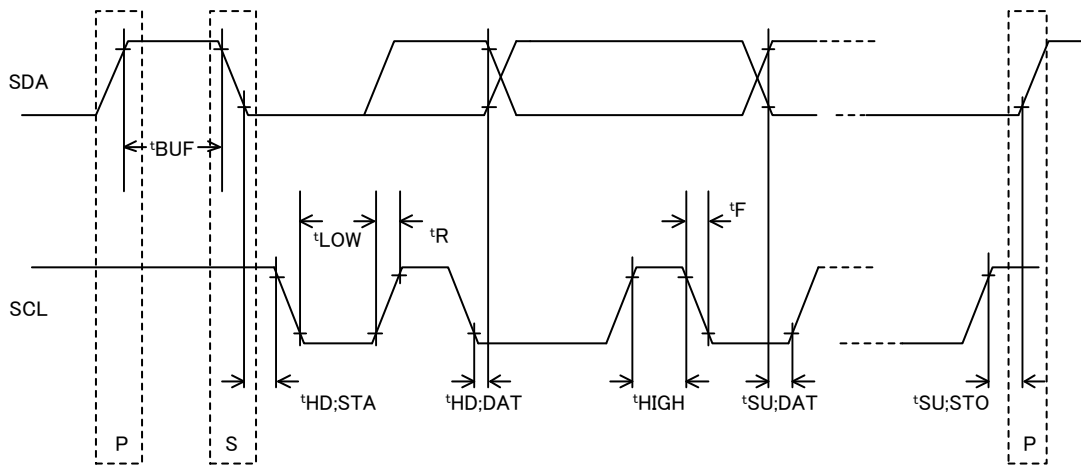
Figure V.11.5 Timing chart
