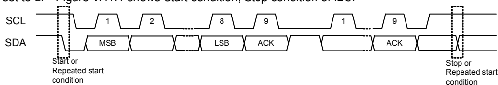
Figure V.11.1 I2C start, stop condition
