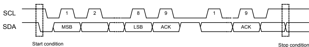
Figure V.11.1 I2C start, stop condition
