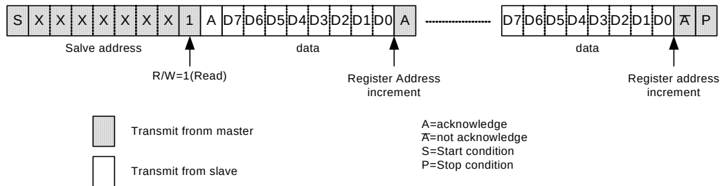
Fig. 10 Readout protocol
