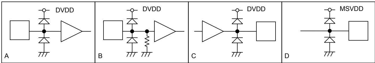
Fig.4. Equivalent Schematics
