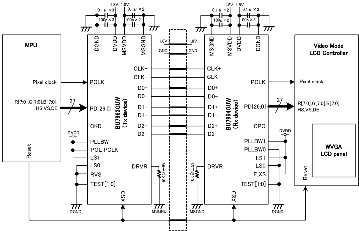
Fig.15. Application Circuit
