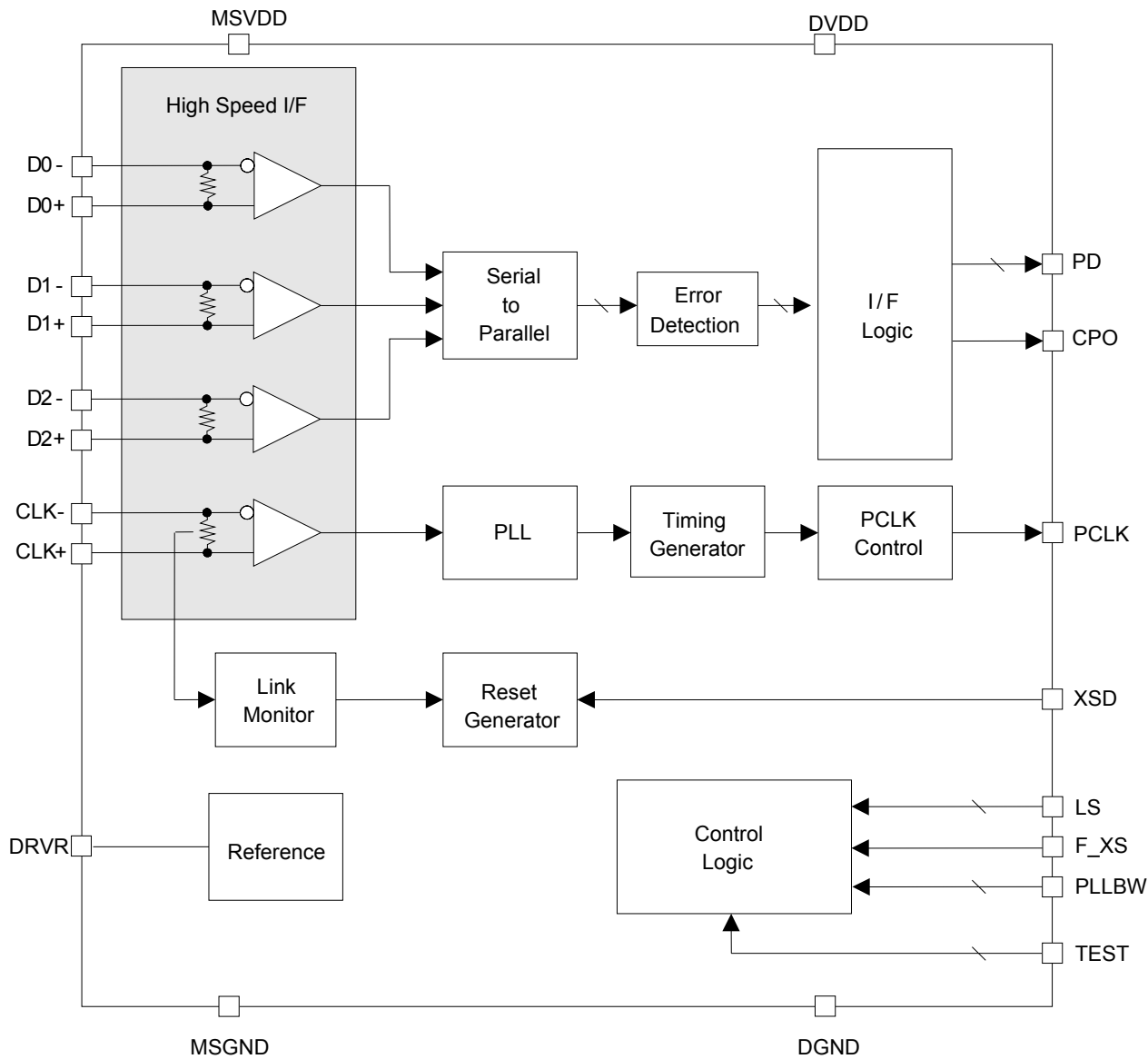
Fig.2. Block Diagram
