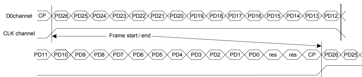
Fig.6. MSDL3 Protocol for 1-channel Data (27-bit)
