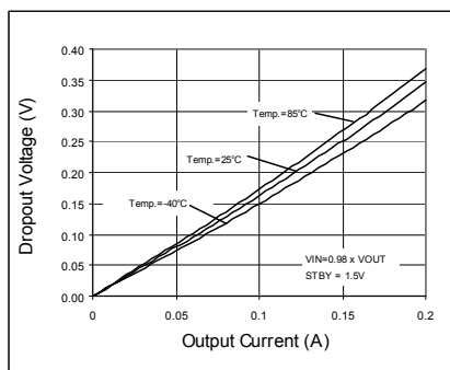
Fig. 43 Dropout Voltage
