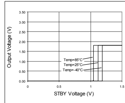
Fig. 74 STBY Threshold
