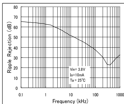
Fig. 49 Ripple Rejection VS Freq.
