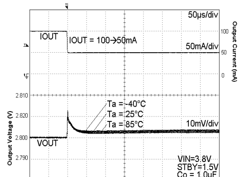
Fig. 55 Load Response
