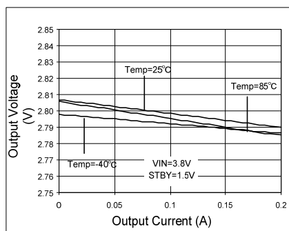
Fig. 46 Load Regulation
