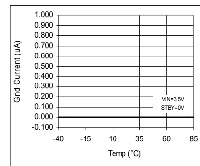
Fig. 106 IGND vs. Temp (STBY)
