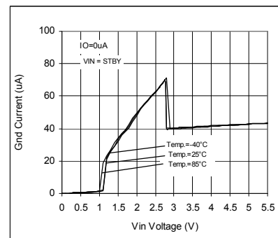
Fig. 42 Circuit Current IGND
