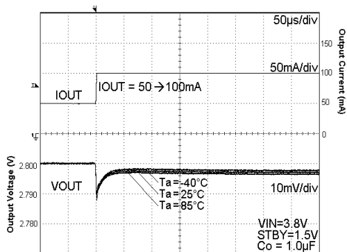
Fig. 54 Load Response
