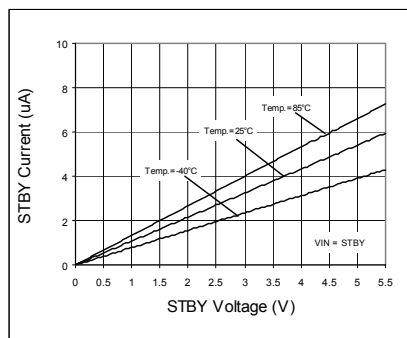
Fig. 44 STBY Input Current
