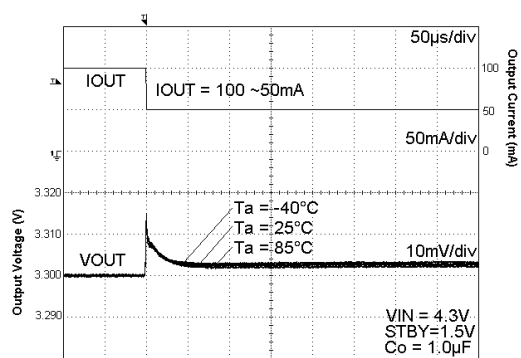
Fig. 29 Load Response
