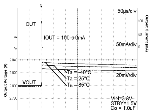
Fig. 53 Load Response
