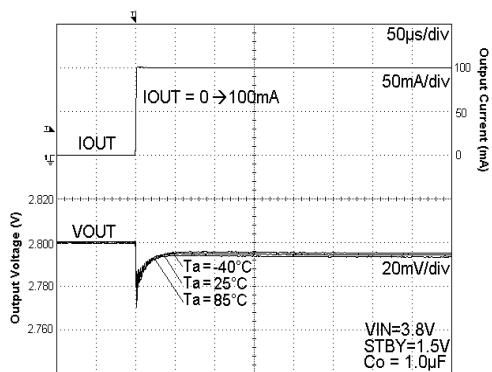
Fig. 52 Load Response
