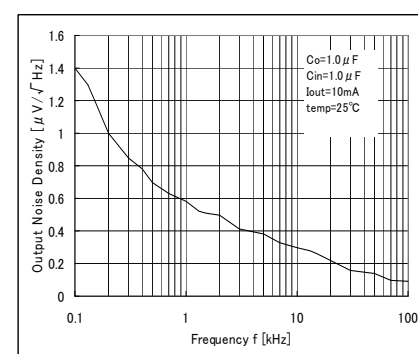
Fig. 51 Output Noise Spectral Density VS Freq.
