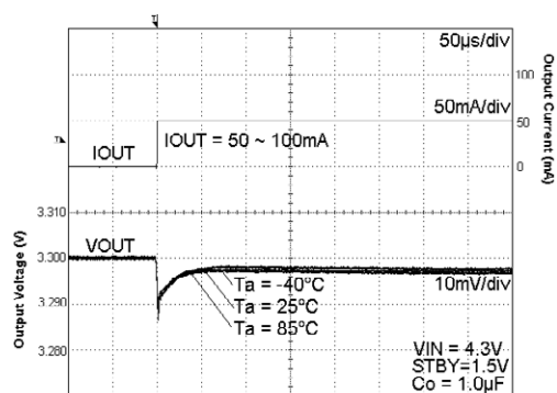
Fig. 28 Load Response
