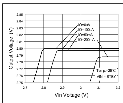
Fig. 41 Line Regulation
