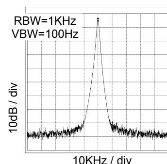
Fig.18 36.9MHz Spectrum VDD=3.3V, at CL=15pF
