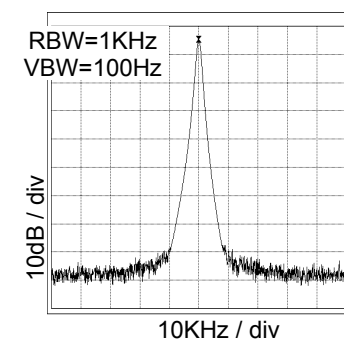
Fig.21 18.4MHz Spectrum VDD=3.3V, at CL=15pF
