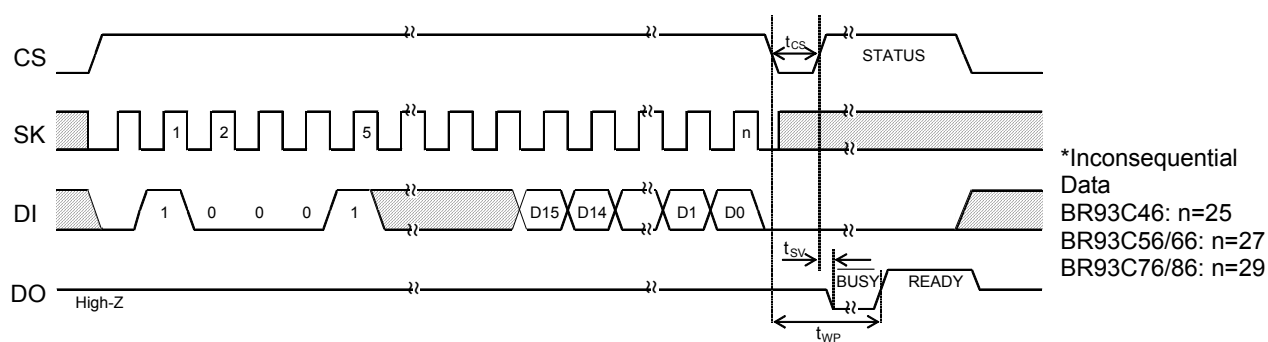
Figure 8: WRAL Sequence
