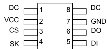
8-lead SOIC Rotated (1K JEDEC only)
