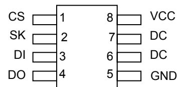
8-lead SOIC
