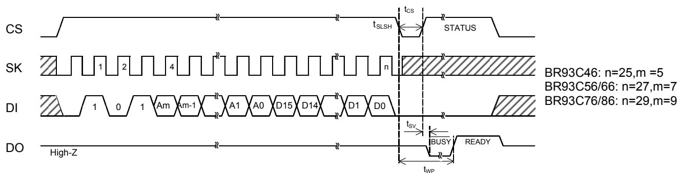
Figure 7: WRITE Sequence
