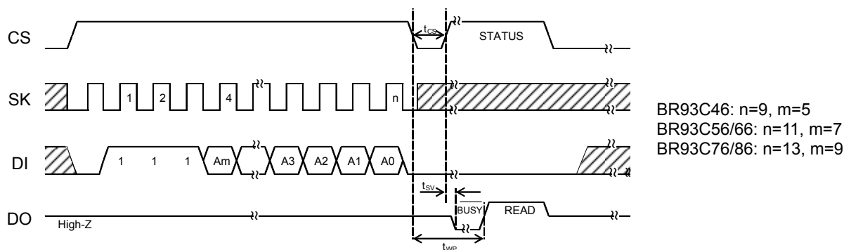
Figure 9: ERASE Sequence
