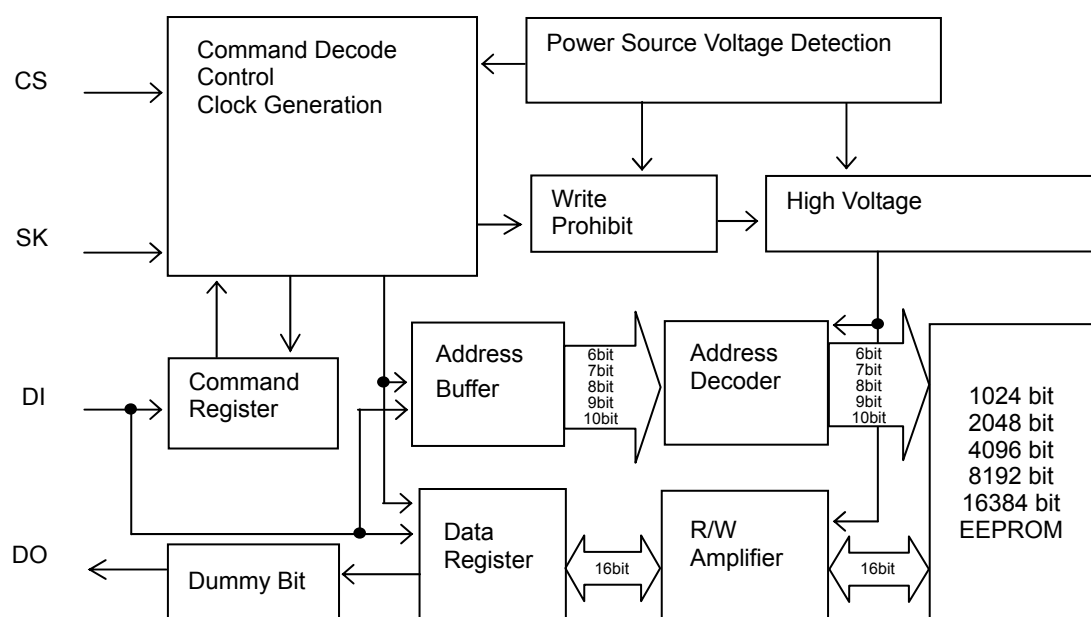
Figure 2: Block Diagram
