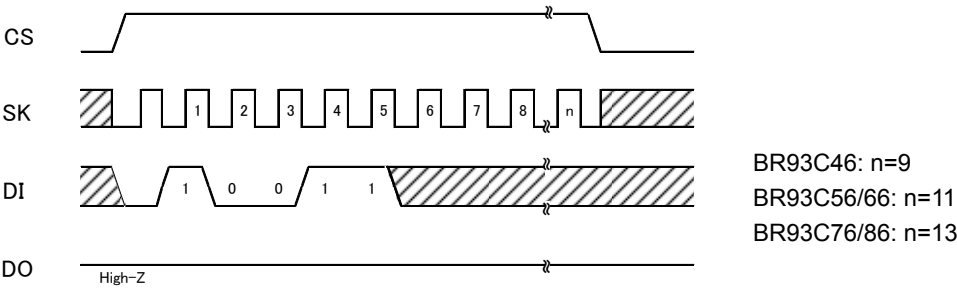
Figure 5: EWEN Sequence
