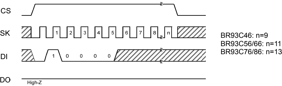
Figure 6: EWDS Sequence
