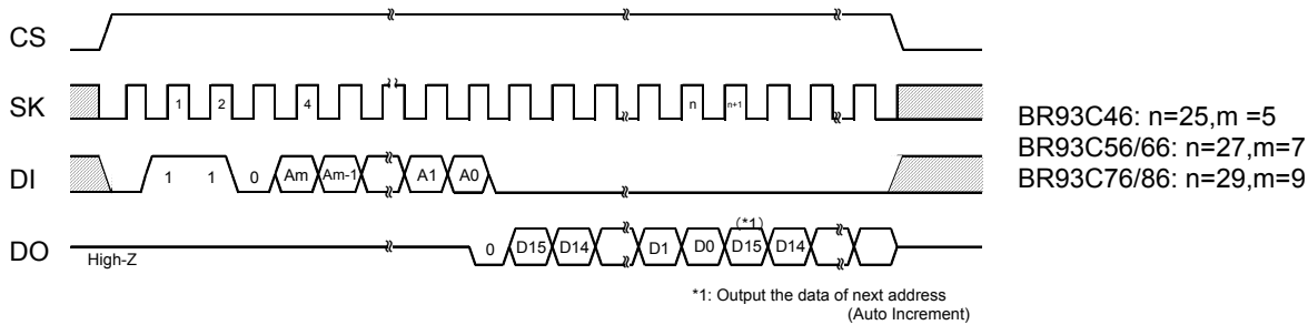
Figure 4: READ Sequence
