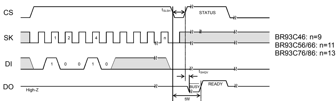
Figure 10: ERAL Sequence.
