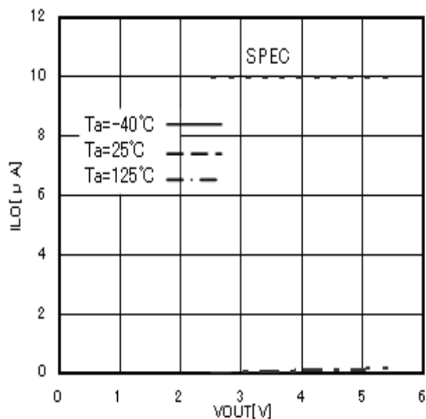
Fig.11 Output leak current ILO (SO)( V_{CC}=5.5V )
