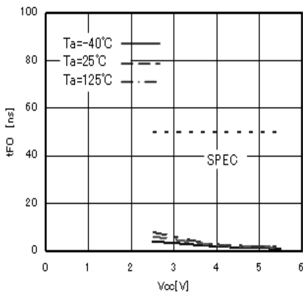
Fig.31 Output fall time t_{FO}
