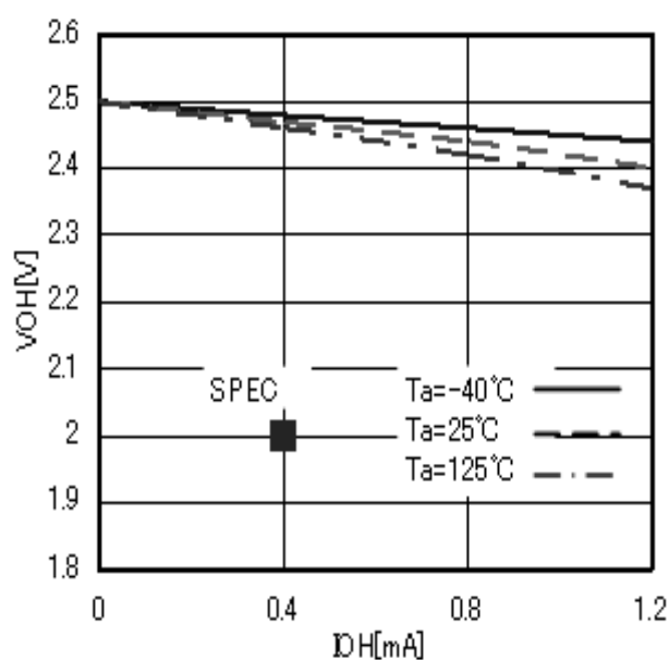
Fig.9 "H" output voltage V_{OH} - I_{OH} ( V_{CC}=2.5\text{V} )
