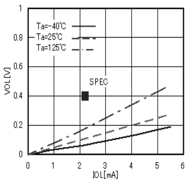
Fig.8 "L" output voltage V_{OL} - I_{OL} ( V_{CC}=2.5\text{V} )
