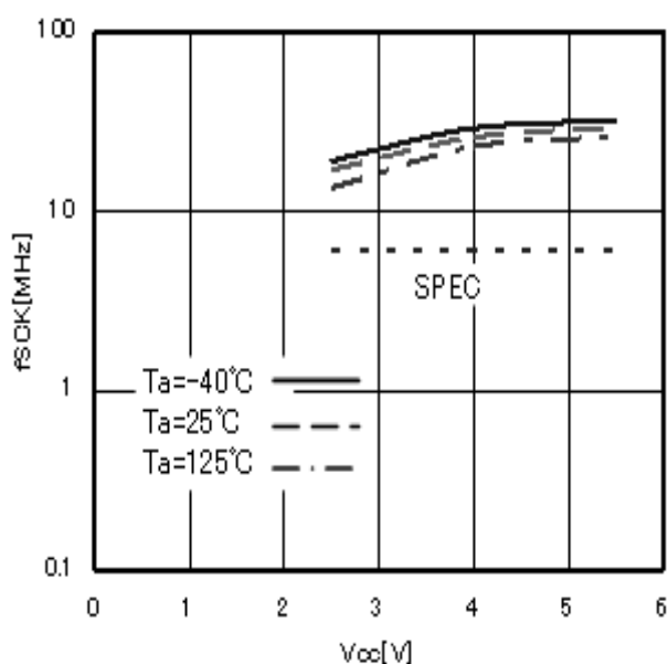
Fig.15 SCK frequency f_{SCK}
