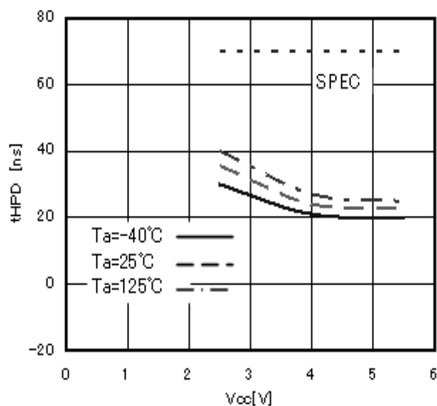
Fig.29 Time from HOLDB to output change t_{HPD}
