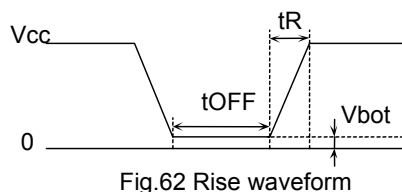
Fig.62 Rise waveform
