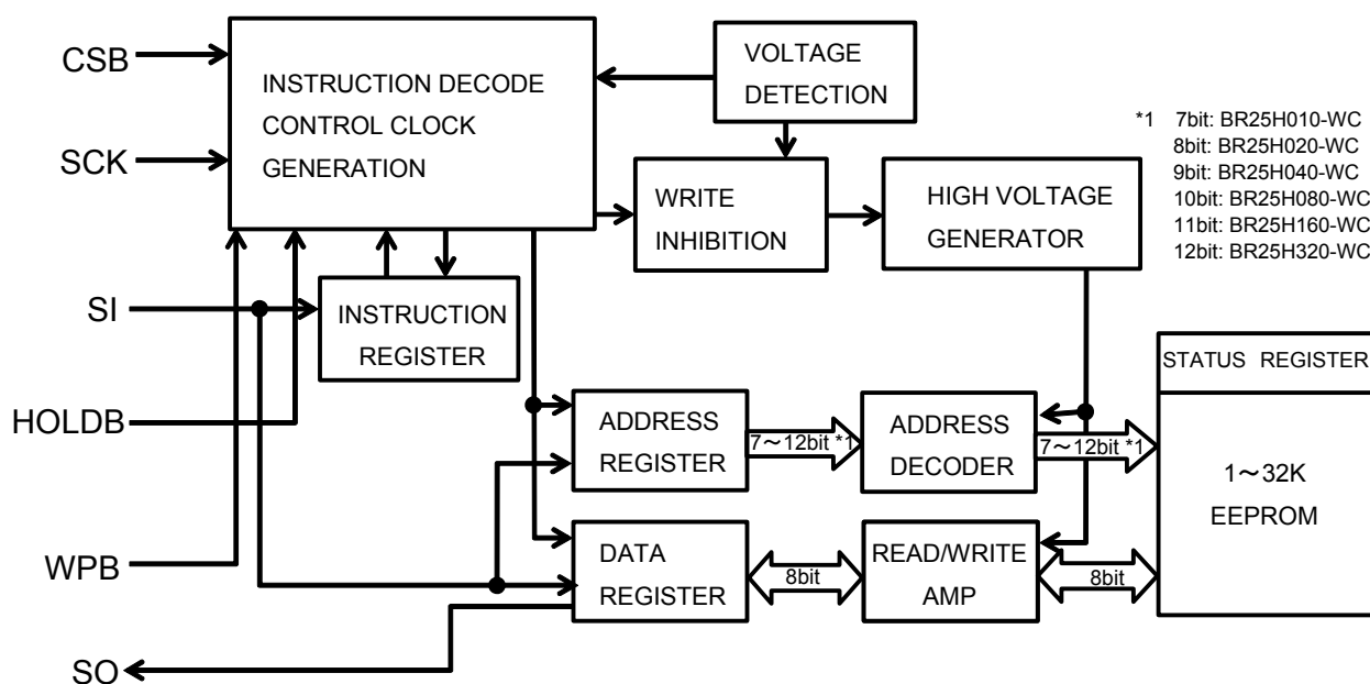
Fig.4 Block diagram
