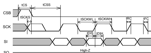
Fig.1 Input timing
