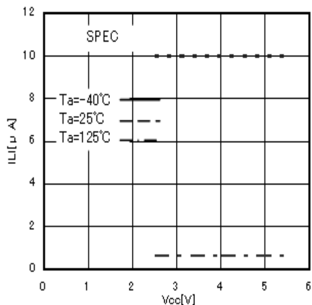
Fig.10 Input leak current ILI (CSB,SCK,SI,HOLDB,WPB)
