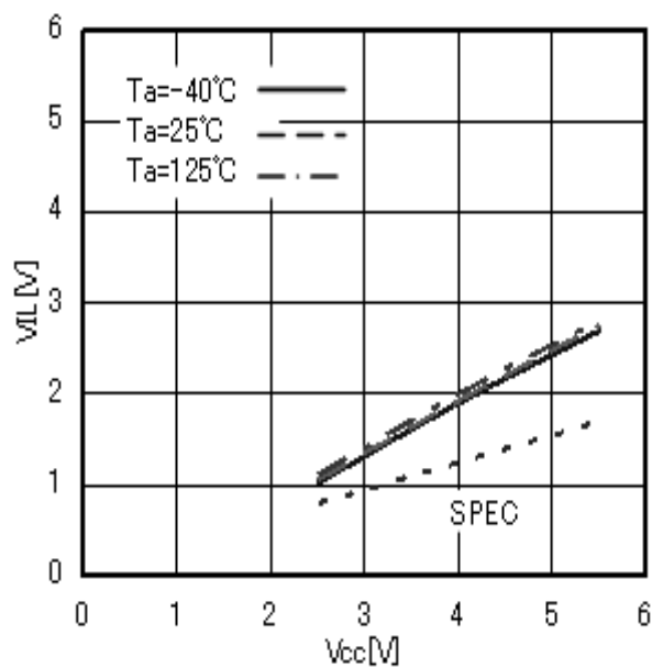
Fig.7 "L" input voltage V_{IL} (CSB,SCK,SI,HOLDB,WPB)
