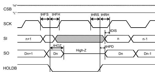
Fig.3 HOLD timing
