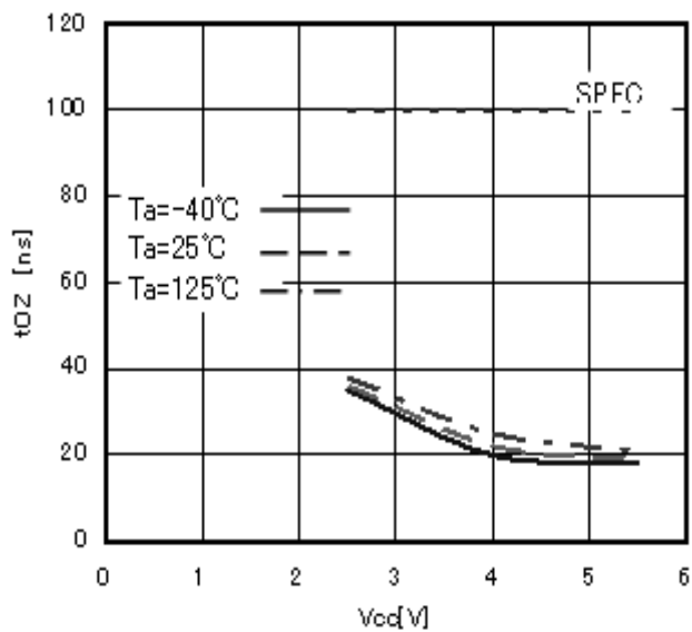
Fig.25 Output disable time t_{OZ}
