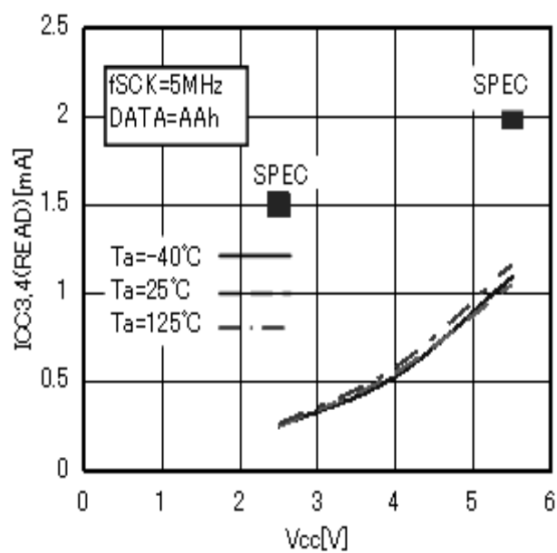
Fig.13 Consumption Current at READ operation ICC3,4
