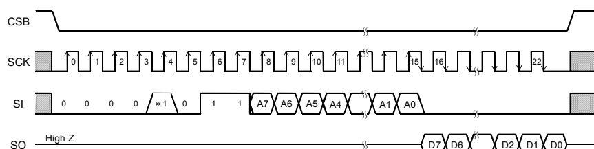
Fig.35 Read command (BR25H010/020/040-WC)
