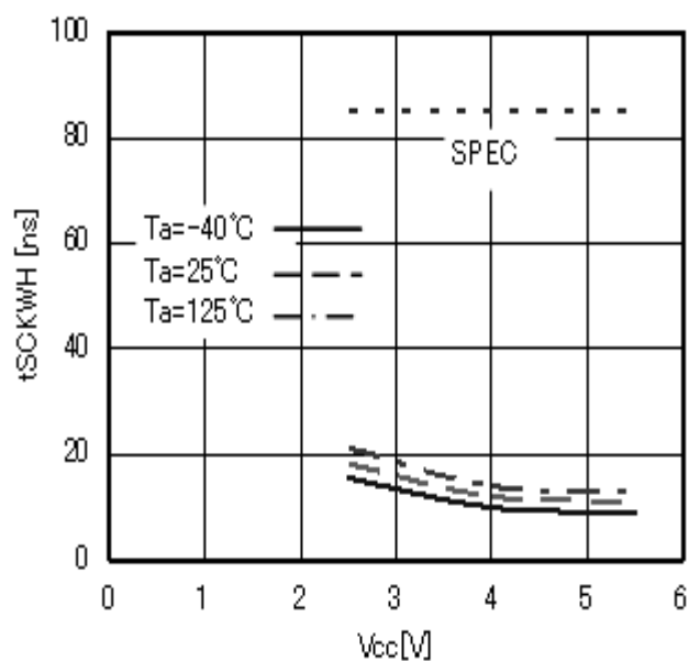
Fig.16 SCK high time t_{SCKWH}
