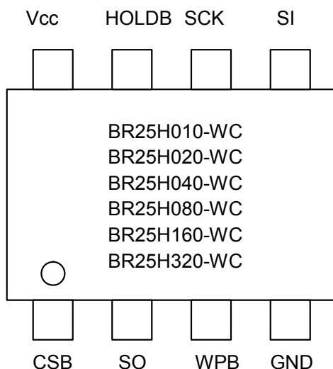
Fig.5 Pin configuration
