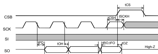
Fig.2 Input / Output timing
