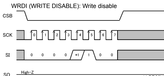
Fig.34 Write disable
