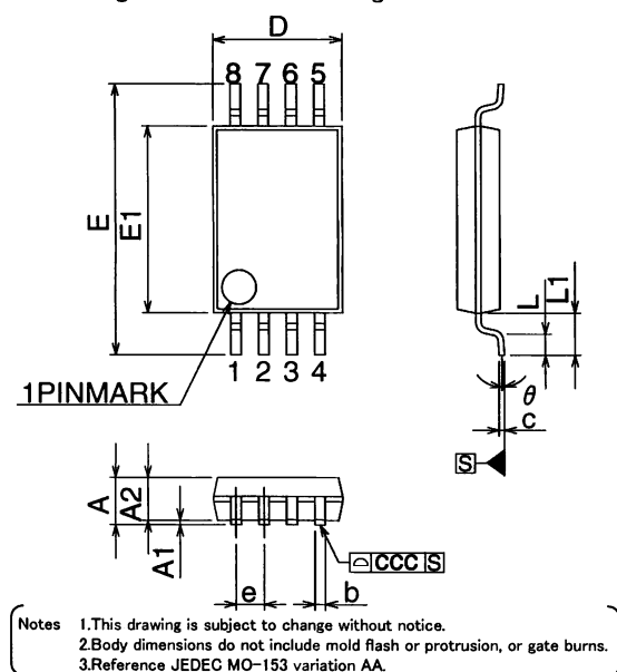
Fig.-5 TSSOP Package Outline
