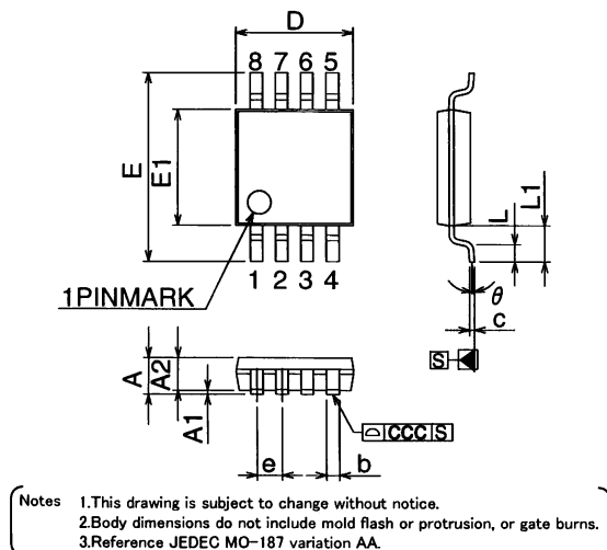
Fig.-6 TSSOP 3 x 3mm² Package Outline
