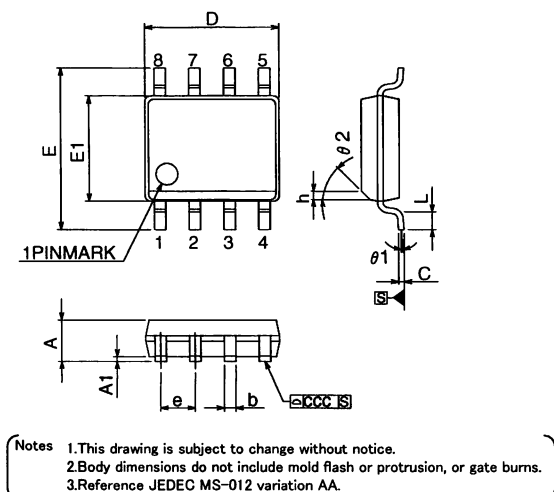
Fig.-4 SO8 narrow Package Outline
