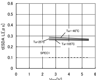
Fig.31 Noise removal valid time t(\text{SDA L})
