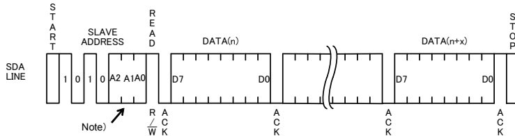
Fig.45 Sequential read cycle (in the case of current read cycle)
