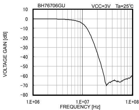
Fig. 25 Frequency Characteristic
