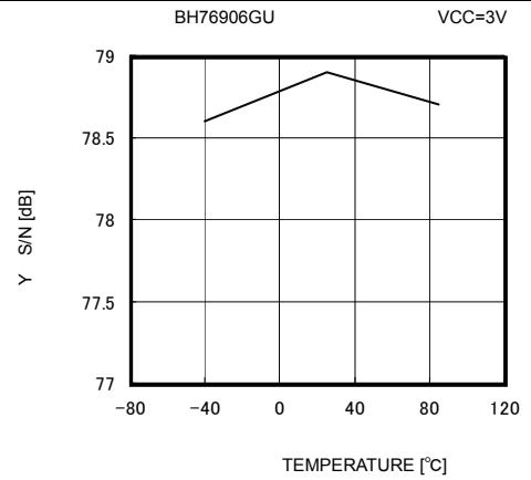
Fig.48 Y S/N vs Ambient Temperature
