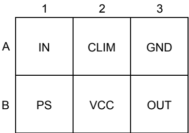
Fig.22 BH6453GUL Pin Arrangement (Top View)
