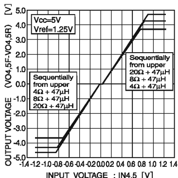
Fig. 19 CH 4 , 5 l / O characteristic : Ta=-40°C
