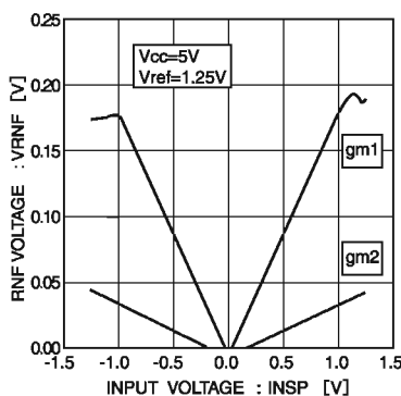
Fig. 24 Spindle driver I/O characteristic : T_a=90^{\circ}\text{C}
