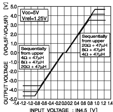
Fig. 20 CH 4 , 5 l / O characteristic : Ta=27°C
