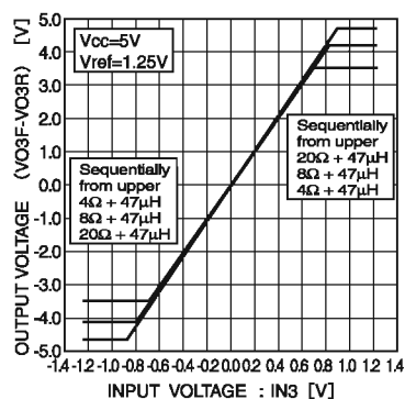
Fig. 18 CH3 I / O characteristic : Ta=90°C
