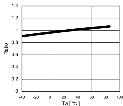
Fig.8 IOU Temperature dependency ( 100 lx )
