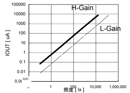
Fig.3 Illuminance - IOU Characteristics
