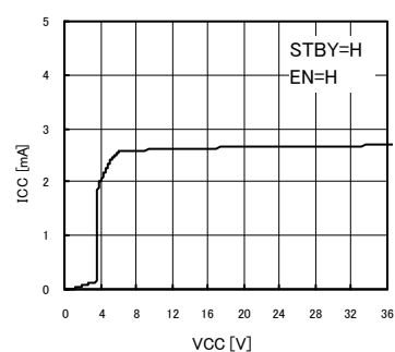
Fig.4-3 Circuit electric current (at the time of operating mode)
