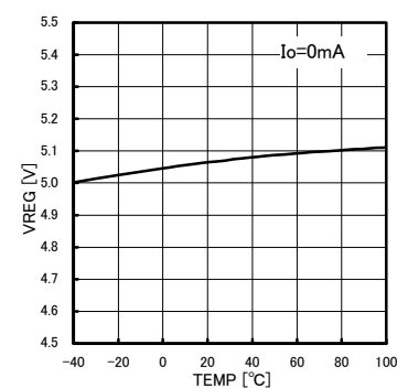
Fig.4-8 VREG temperature characteristic
