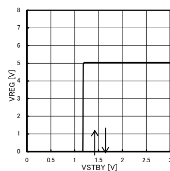
Fig.4-9 STBY Threshold voltage
