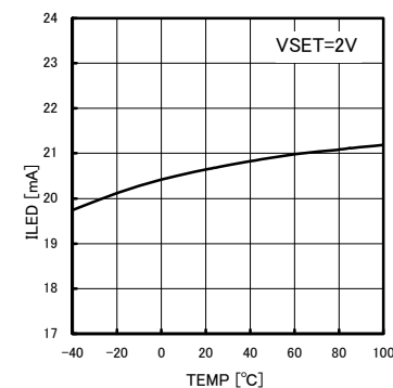
Fig.4-6 Constant electric current temperature characteristic
