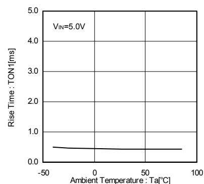
Fig.20 Output rise time
