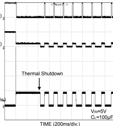
Fig.36 Thermal shutdown 1Ω load connected at enable
