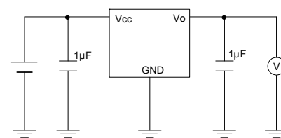
Measurement Circuit of Fig.9 and Fig.18
