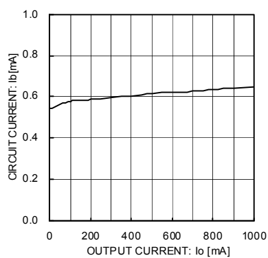
Fig.8 Circuit Current ( I_o=0\text{mA} \rightarrow 1000\text{mA} )
