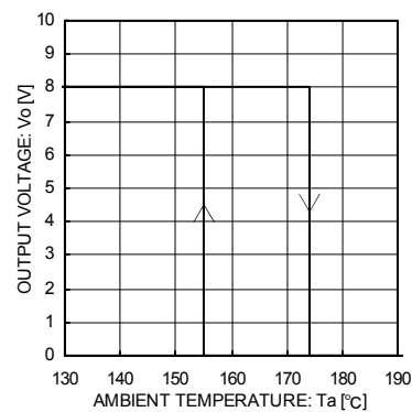
Fig.9 Thermal Shutdown Circuit Characteristics
