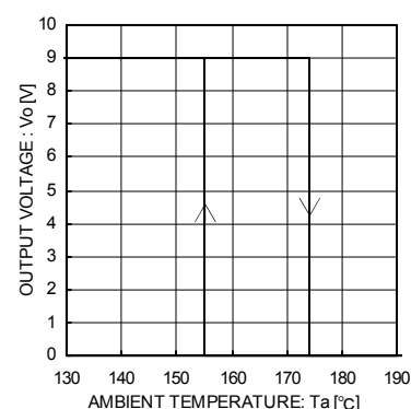
Fig.18 Thermal Shutdown Circuit Characteristics
