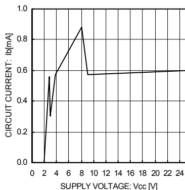
Fig.1 Circuit Current
