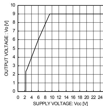
Fig.12 Line Regulation ( I_o=500\text{mA} )
