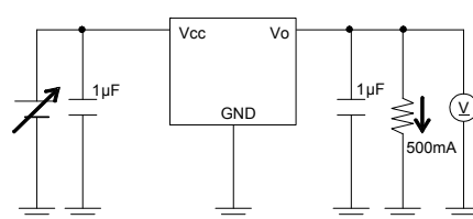
Measurement Circuit of Fig.3 and Fig.12
