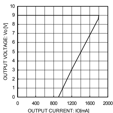
Fig.13 Load Regulation
