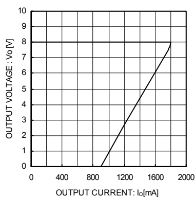
Fig.4 Load Regulation
