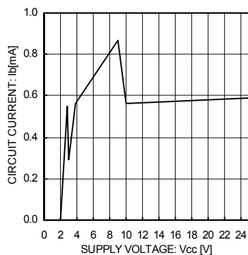
Fig.10 Circuit Current
