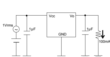
Measurement Circuit of Fig.6 and Fig.15
