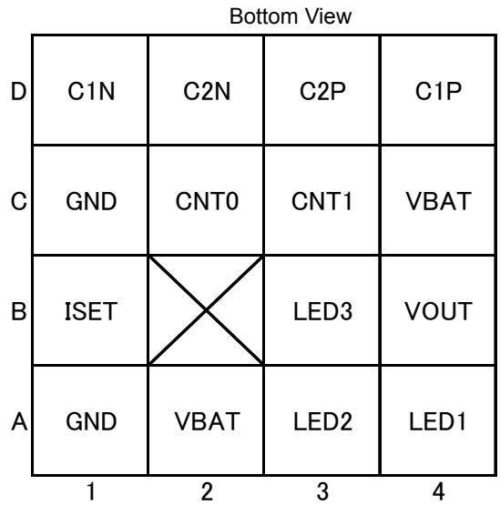
Fig-3. Pin Location
