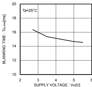
Fig.25 Blanking time
