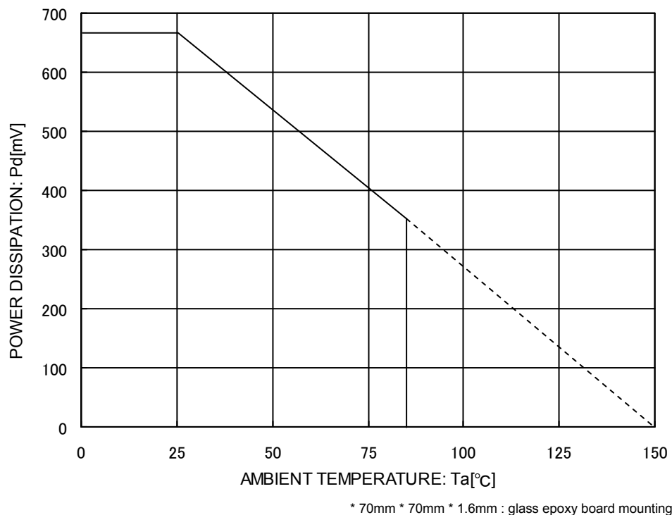
Fig.42 Power dissipation curve (Pd-Ta Curve)
