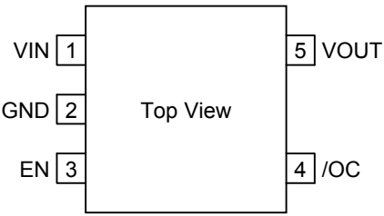
Fig.37 Pin Configuration
