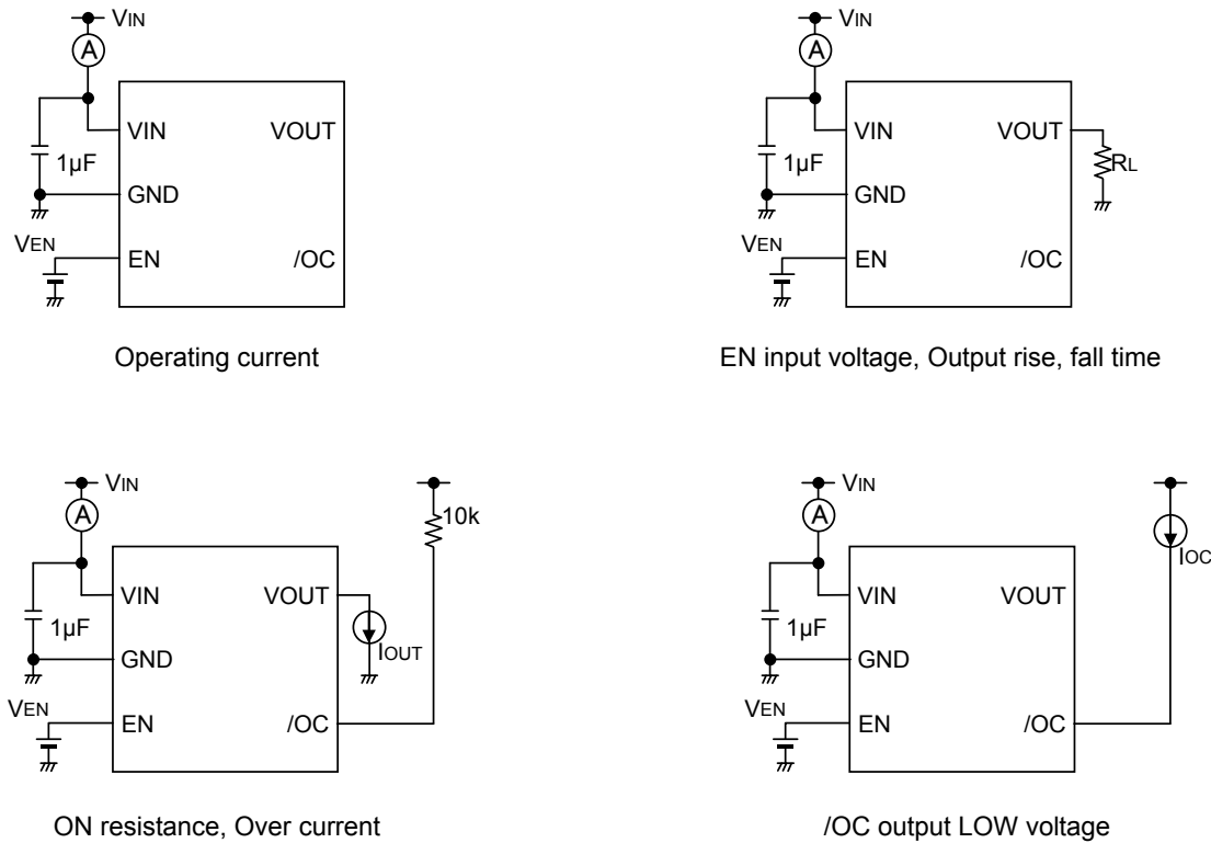
Fig.1 Measurement circuit
