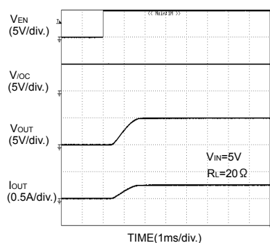
Fig.27 Output rise characteristic
