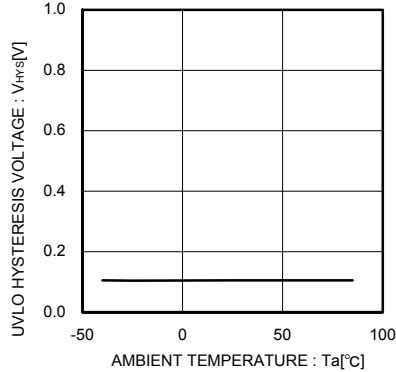
Fig.16 UVLO hysteresis voltage
