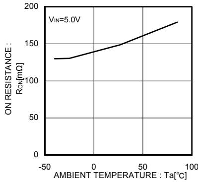
Fig.10 ON resistance
