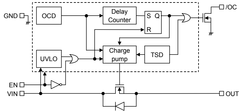
Fig.36 Block diagram
