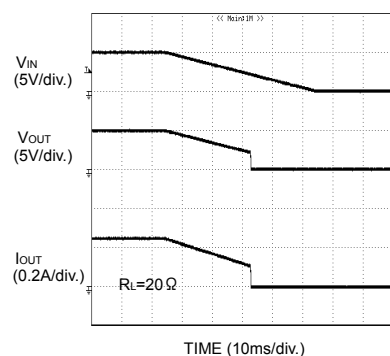
Fig.35 UVLO response V_{IN} Decreasing
