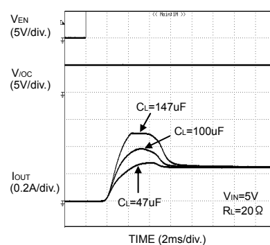
Fig.29. Inrush current response
