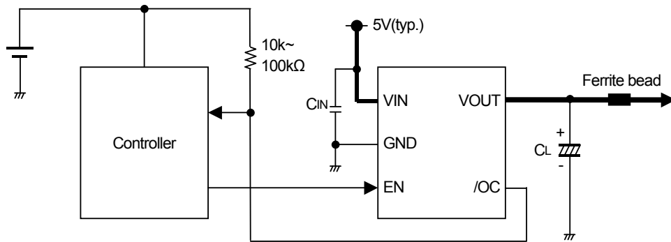
Fig.41 Typical application circuit
