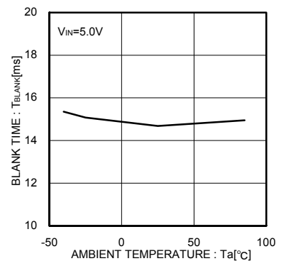
Fig.26 Blanking time
