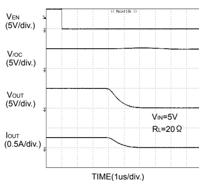
Fig.28 Output fall characteristic
