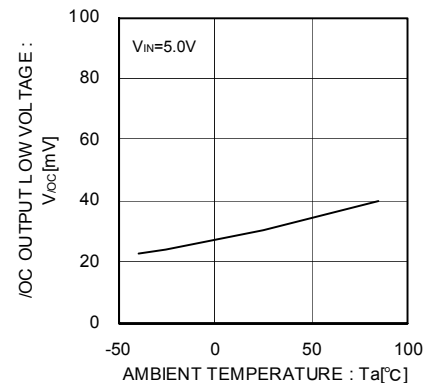
Fig.14 /OC output LOW voltage
