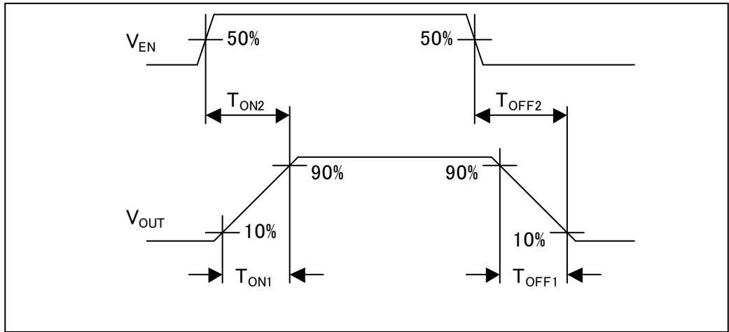
Fig.2 Timing chart at output rise / fall time
