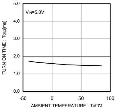
Fig.20 Output turn on time
