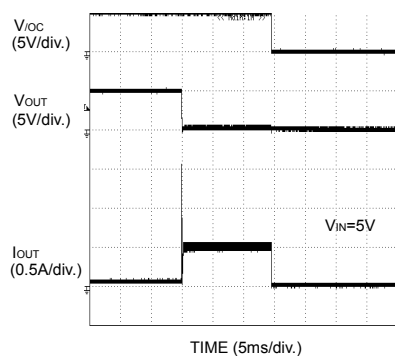
Fig.33 Over current response Output shortcircuit at Enable
