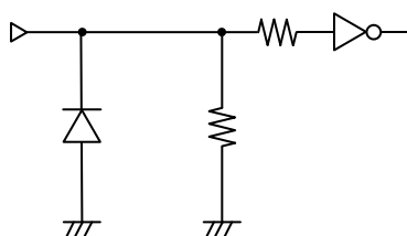
Fig.29 I/O Circuit
