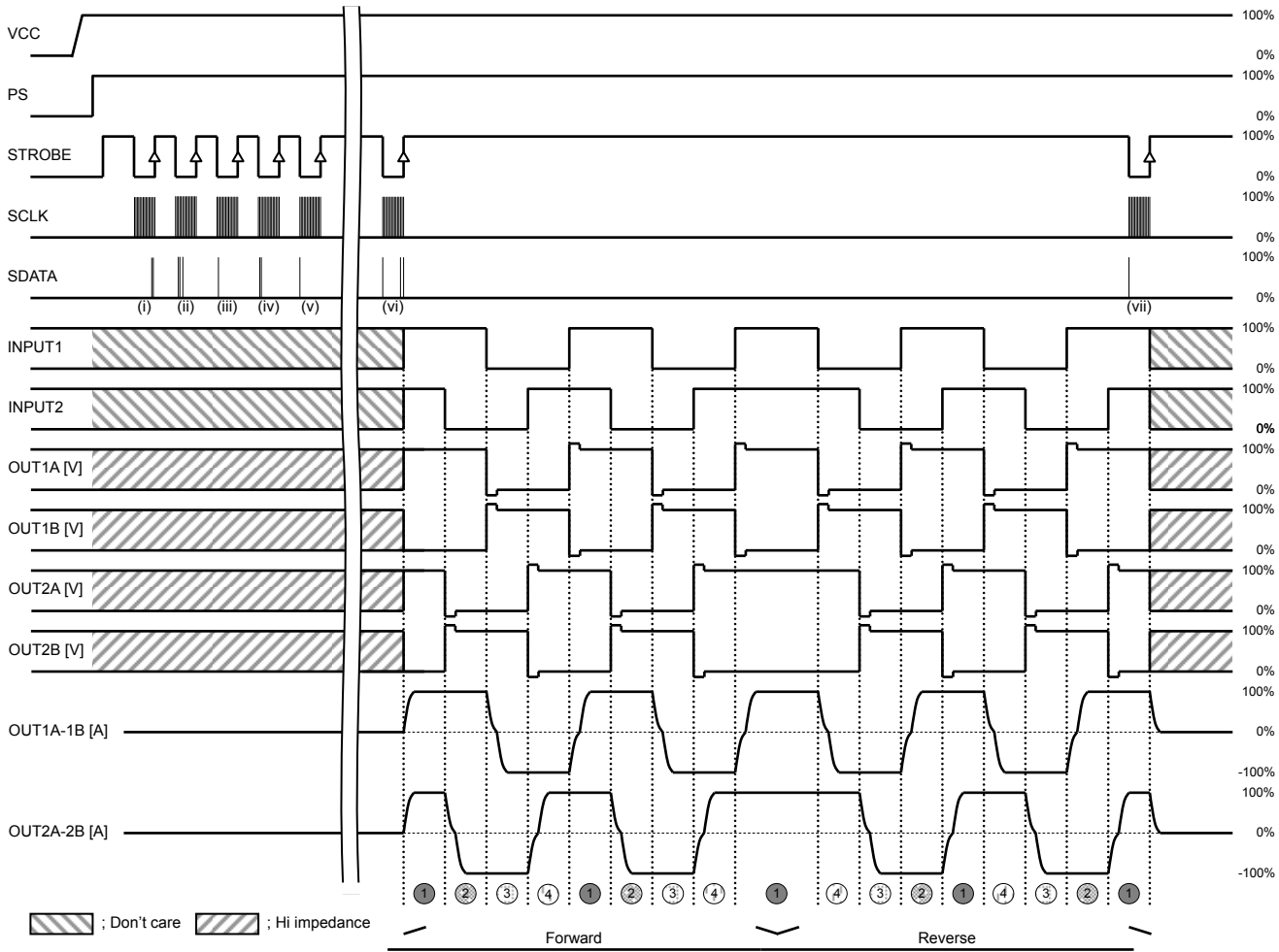
Fig.48 Timing Chart of Stepping Motor Drive
