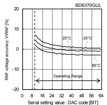
Fig.12 RNF Voltage Accuracy (Const.-Current drive block, RDNFX=1.0Ω, RL=10Ω)
