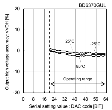
Fig.6 Output High Voltage Accuracy (Const.-Voltage drive block, RL=20Ω)
