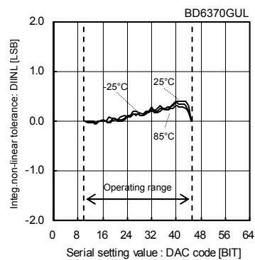
Fig.8 Integral Non-Linear Tolerance (Const.-Current drive block, RDNFX=0.5Ω, RL=10Ω)
