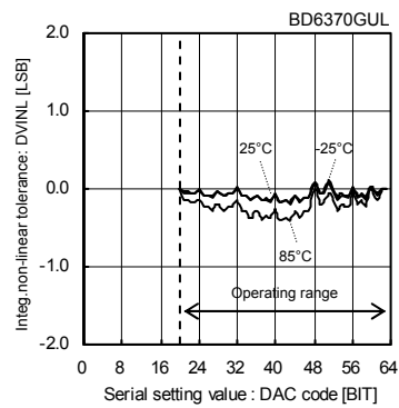
Fig.5 Integral Non-Linear Tolerance (Const.-Voltage drive block, RL=20Ω)
