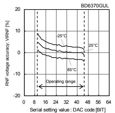
Fig.9 RNF Voltage Accuracy (Const.-Current drive block, RDNFX=0.5Ω, RL=10Ω)
