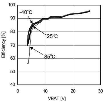
Fig 16. Efficiency 10LEDx6CH
