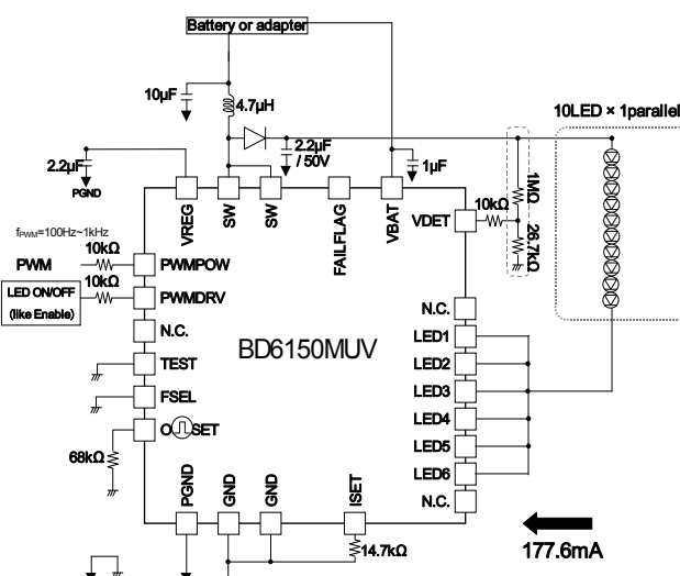
Fig.56 10series \times 1parallel, LED current 177.6mA setting, Switching frequency 1250kHz setting example Power control PWM application
