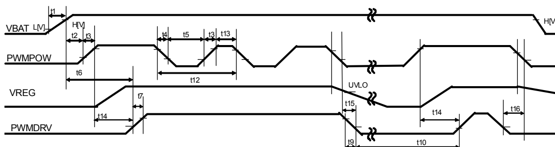
Fig.28 input timing
