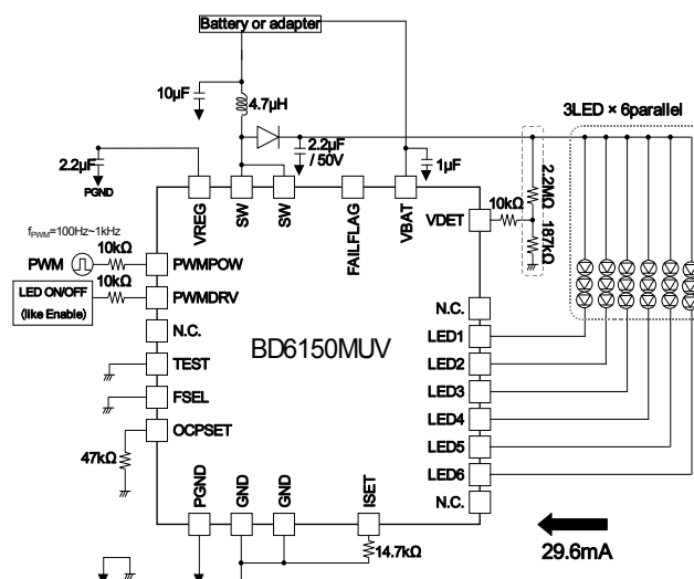
Fig.54 3series \times 6parallel, LED current 29.6mA setting, Switching frequency 1250kHz setting example Power control PWM application
