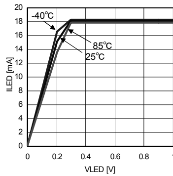
Fig 14. LED Current vs LED Voltage
