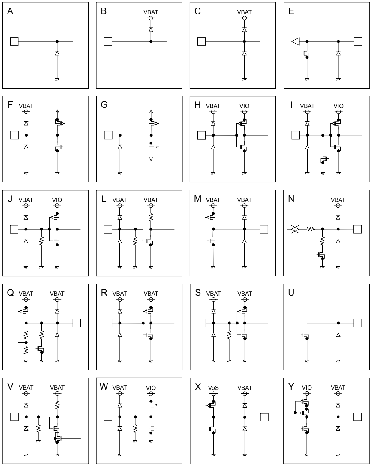
Fig.7 Equivalent Circuit
